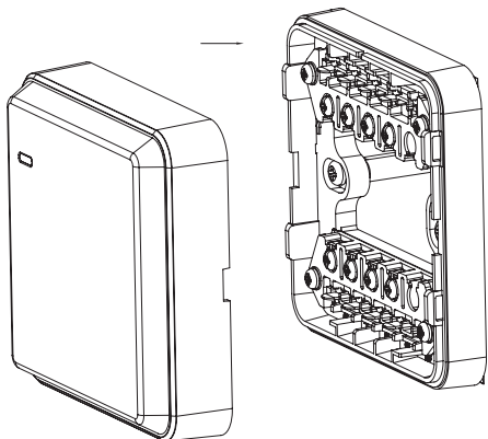
Figure 3-6 Installation (3)
