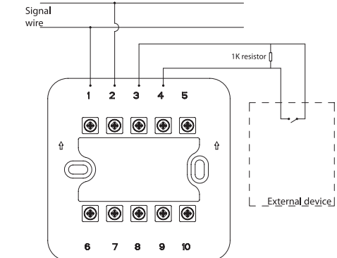
Figure 3-2 Normally open input
