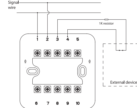
Figure 3-3 Normally closed input
