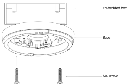
Figure 3-1 Installation (1)
