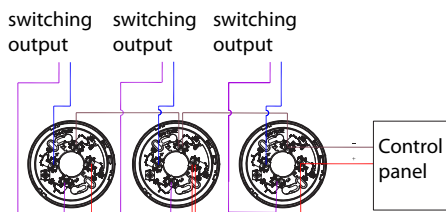
Figure 3-2 Wiring
