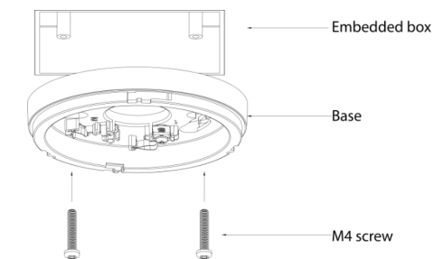
Figure3-1 Installation (1)
