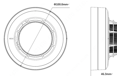
Figure1-1 Dimension [mm (inch)]
